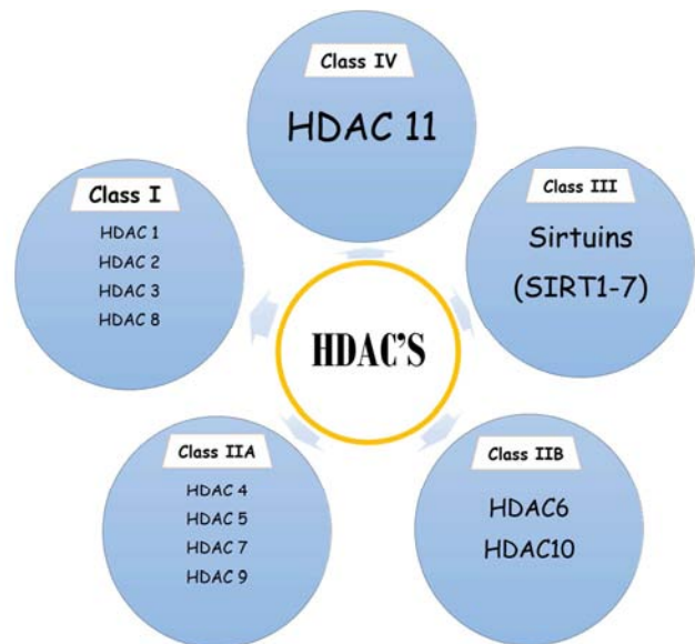
Figure 9. Classification of HDAC's [111].
